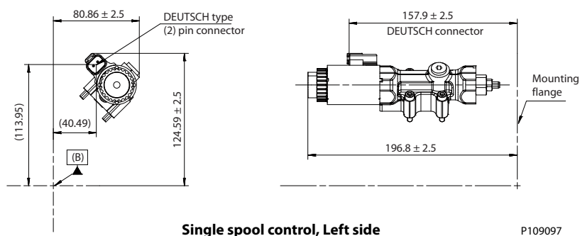
Single spool control, Left side
