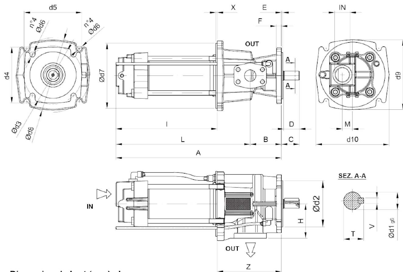
Dimensional chart (mm) - bar
